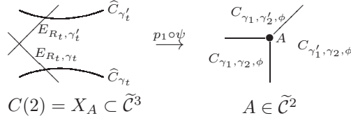
Figure 3. The local picture of A and the fiber X_A = p_1 \circ \psi^{-1}(A) .
