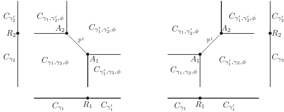
Figure 1. The blowups \tilde{\mathcal{C}}^2 \rightarrow \mathcal{C}^2 along C_{\gamma_1} \times C_{\gamma_2} and C_{\gamma_1} \times C_{\gamma'_2} .
