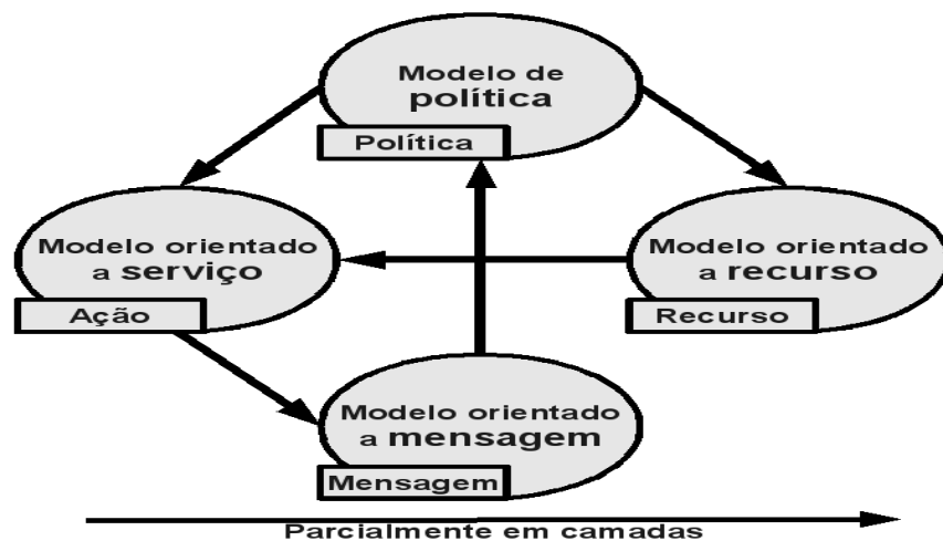
Figura 9: Modelo W3C SOA [W3C 2004].
