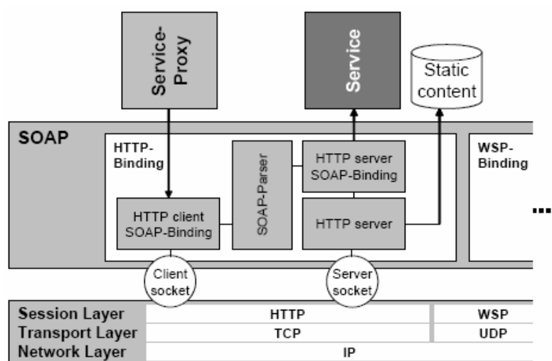
Figura 3.10 – Servidor HTTP-Binding
