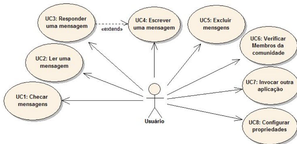
Figura 5.29: Diagrama use/case do software E-mail
