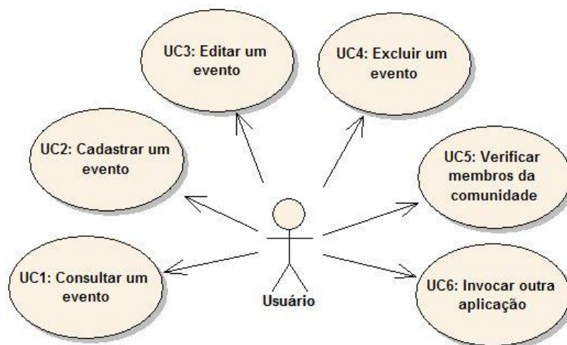
Figura 5.27: Diagrama use/case do software Agenda
