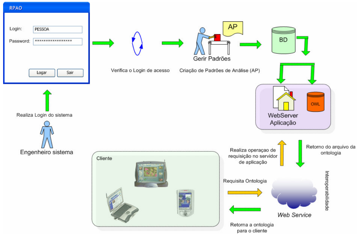
Figura 58: WorkFlow do RPAO.
