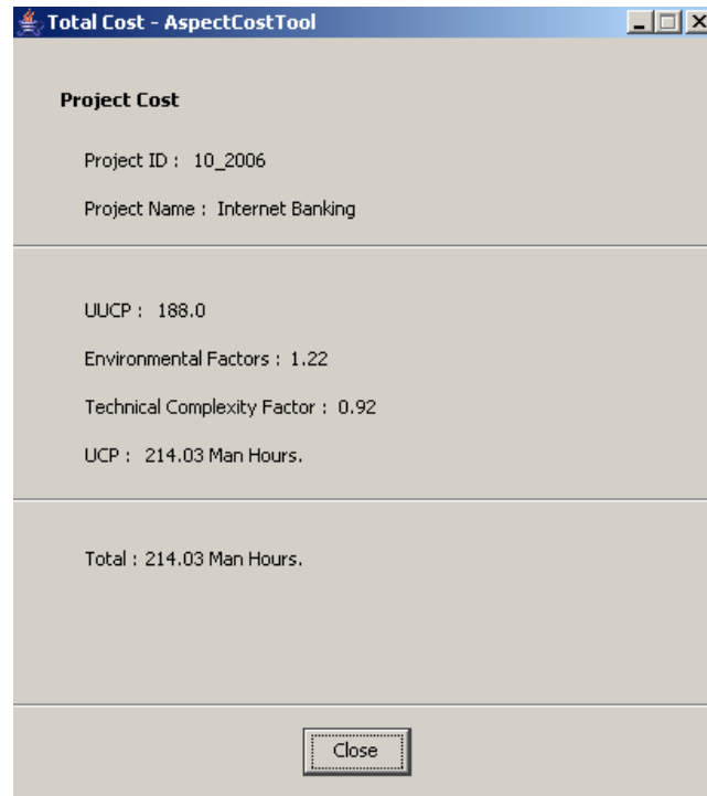
Figura 27 : Custo total Internet Banking
